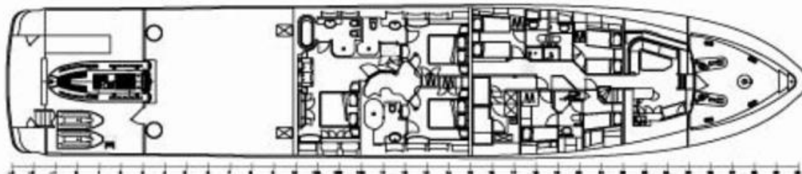
LOWER DECK
